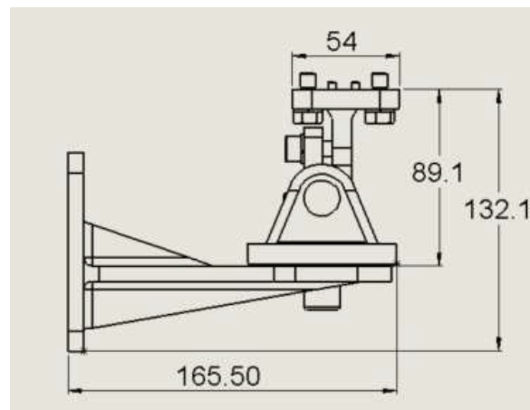
Figure 12 : Tilt mount base – Side View
