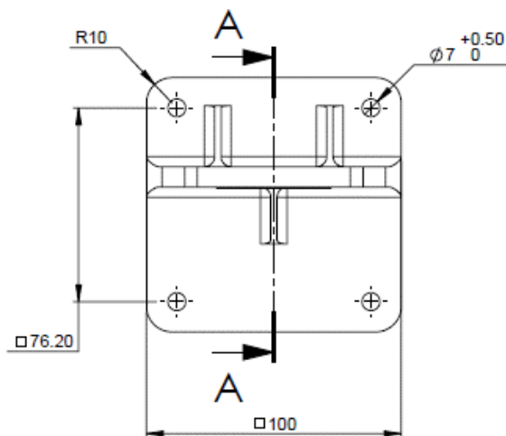
Figure 11 : Tilt Mount Base - Plate View
