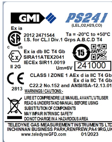
Figure 1-1: Identification Label
